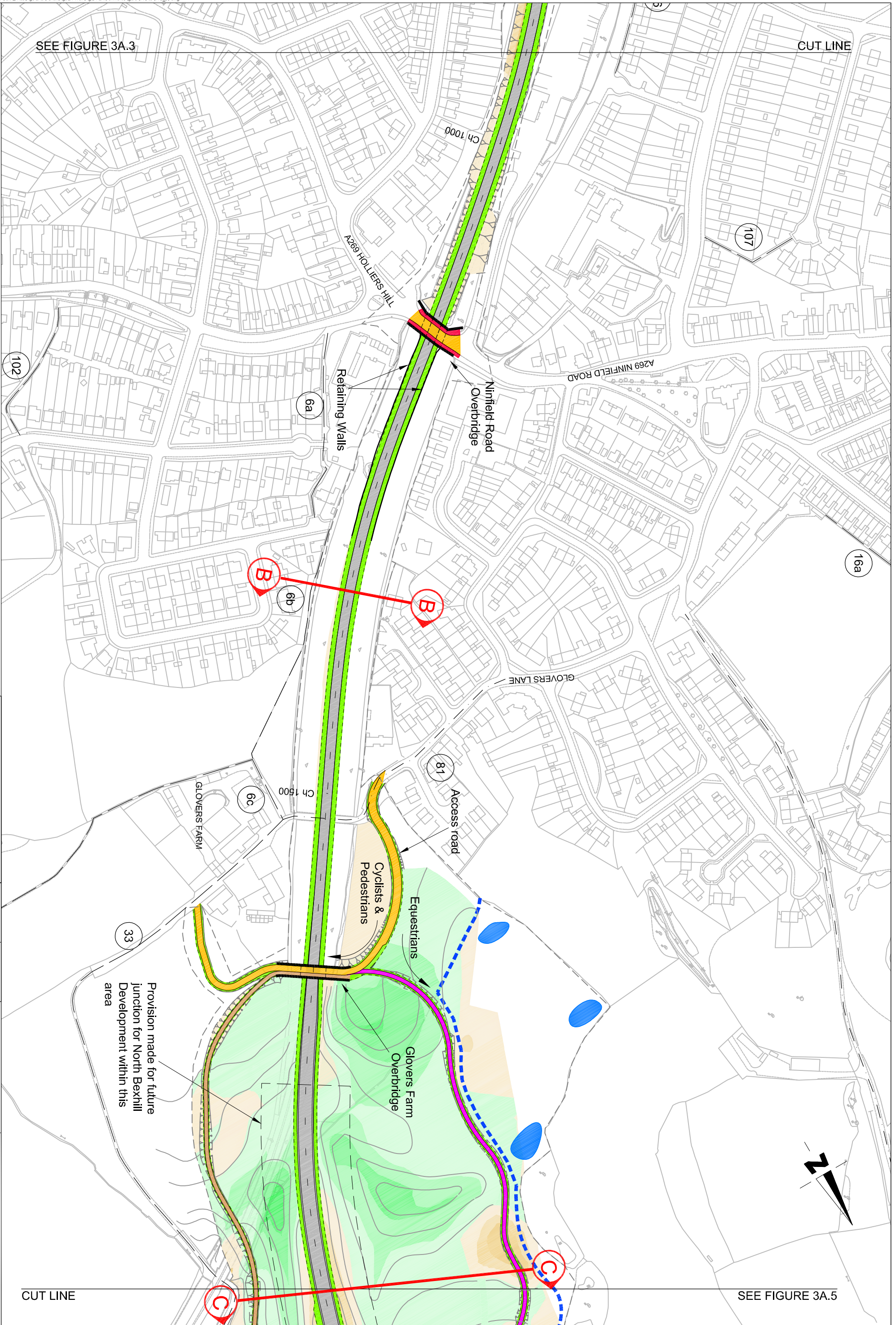
Figure : 3A.4 SCHEME PLAN
